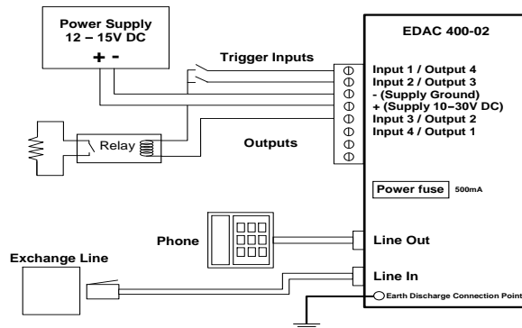
Figure 1: Typical EDAC 400-02 Installation
